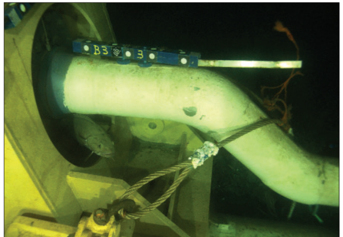
Tee survey. Angles and positions to be determined.
